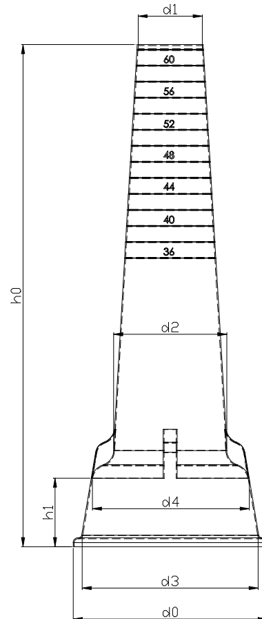
8" Footing Tube
